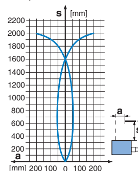
Response curve:
