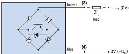
Diagram 7 2-wire DC normally open (N.O.)
