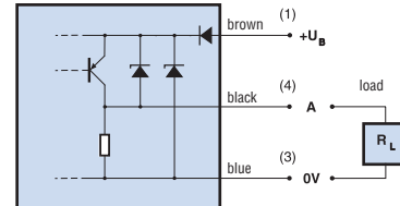
PNP normally open (N.O.) / normally closed (N.C.)
