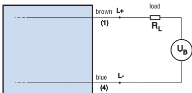
Diagram 4 2-wire NAMUR
