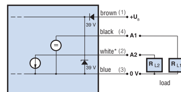
Diagram 5 Analog output
